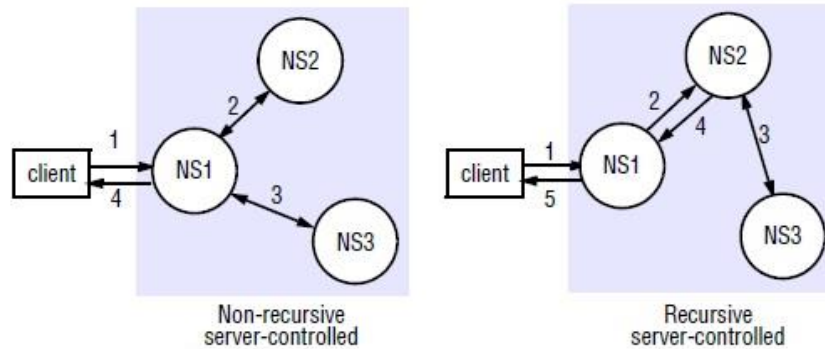
A name server NS1 communicates with other name servers on behalf of a client
