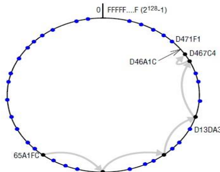
The dots depict live nodes. The space is considered as circular: node 0 is adjacent to node (2^{128}-1) . The diagram illustrates the routing of a message from node 65A1FC to D46A1C using leaf set information alone, assuming leaf sets of size 8 ( \neq 4 ). This is a degenerate type of routing that would scale very poorly; it is not used in practice.
