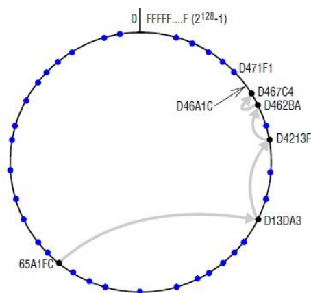
Routing a message from node 65A1FC to D46A1C. With the aid of a well-populated routing table the message can be delivered in \sim \log_{16}(N) hops.
