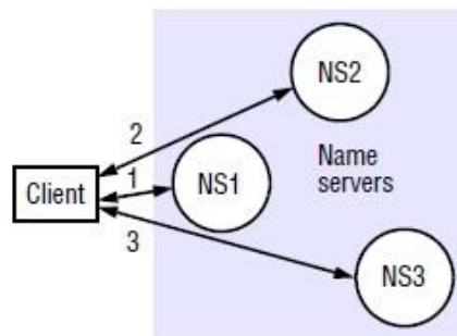
A client iteratively contacts name servers NS1–NS3 in order to resolve a name
